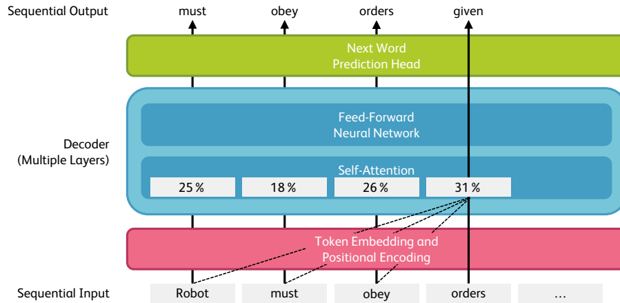
Figure 7.1: Simplified architecture of a generative pretrained transformer (GPT) (source: based on Alammari (2019))
