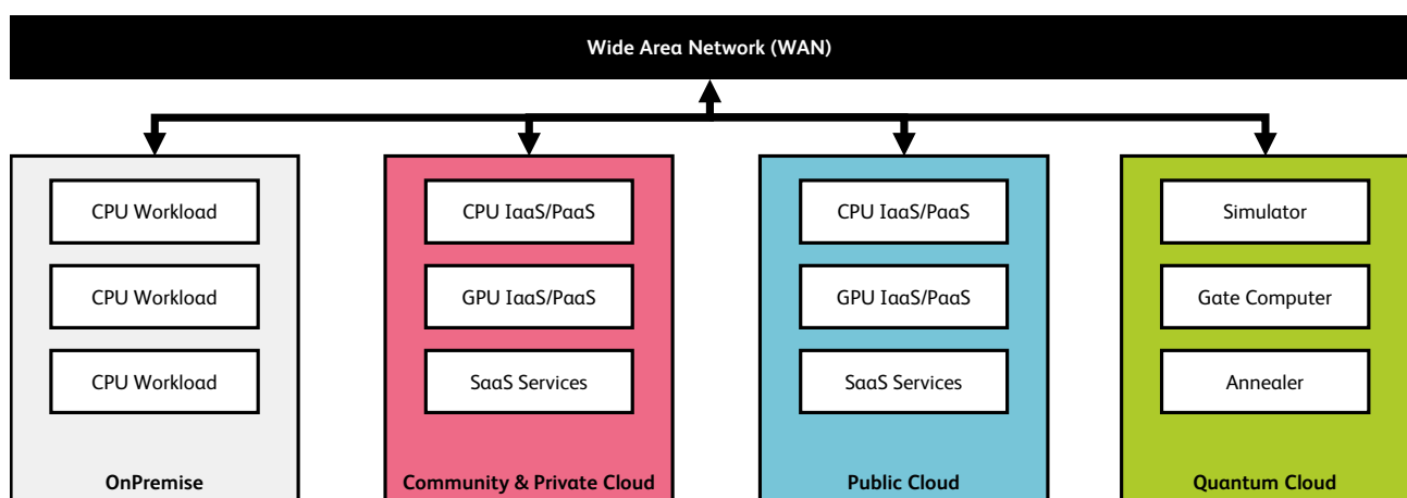
Figure 9.2: Quantum computing as part of a multi-cloud platform
