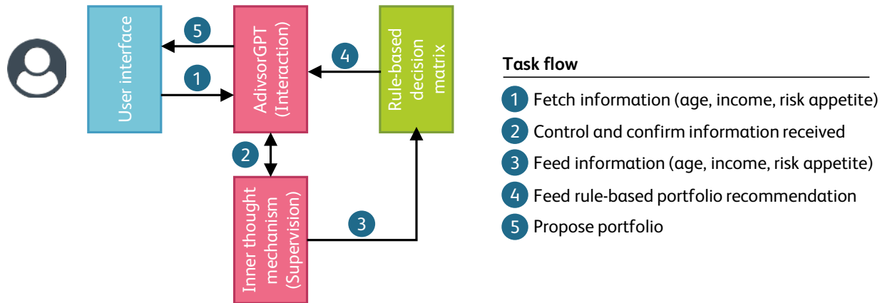
Figure 7.2: General architecture of the prototype and corresponding task flow
